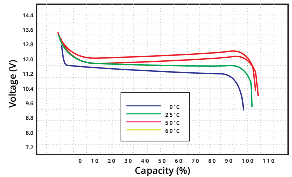
Discharge at -C/2 @ various temperatures
