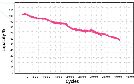
Lifetime at 0.5C, 80% DoD @ 25°C
