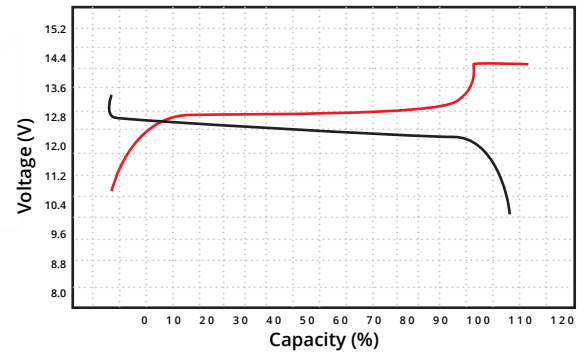
Charge/Discharge at -C/2 @ 25°C
