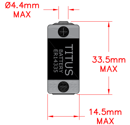
Standard Termination
