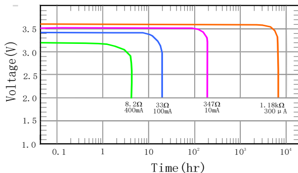
Discharge Characteristics at 23±2°C
