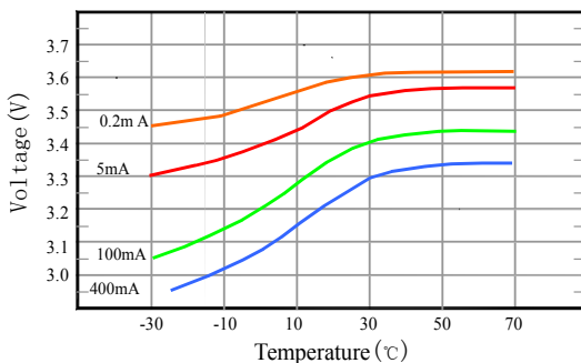
Voltage VS. Temperature
