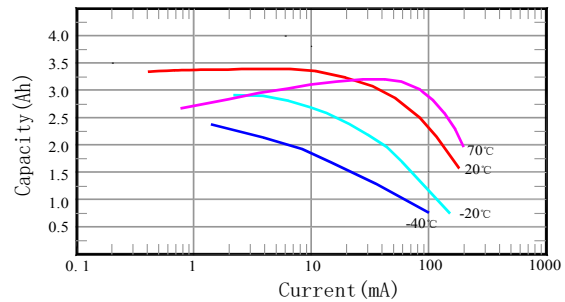
Capacity VS. Current
