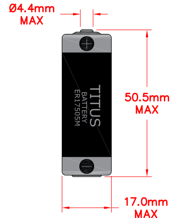
Standard Termination
