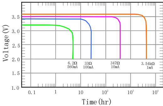
Discharge Characteristics at 23±2°C
