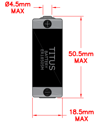
Standard Termination
